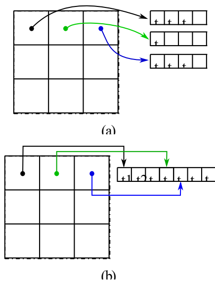
Figure 2: Dynamic array versus ragged array - 3 \times 3 uniform grid using dynamic arrays (a) versus ragged array (b). Only the memory related to the first row of the grid is shown. Source: [25]
