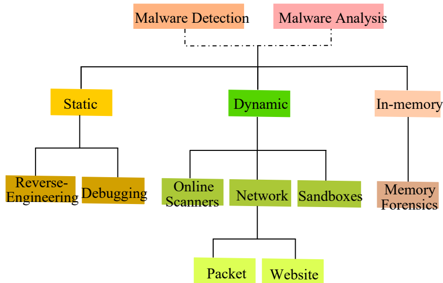
Figure 4. Malware Detection and Analysis Tools
