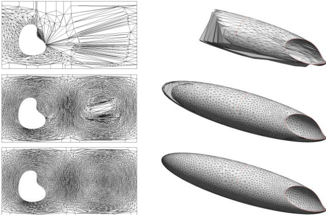
Figure 14: Local mesh modifications with irregular points.
