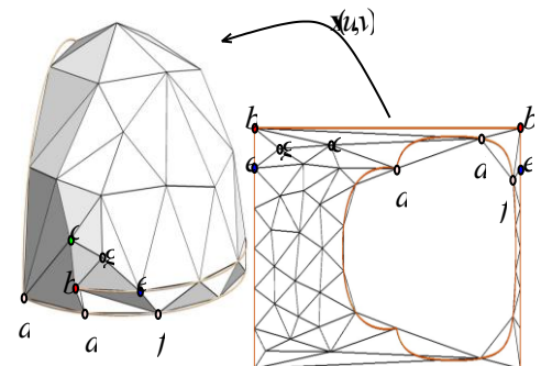
Figure 4: Parameter plane of a sphere. We consider an edge (a,b,c) with c positioned anywhere in the parameter plane. The g in 3D.
