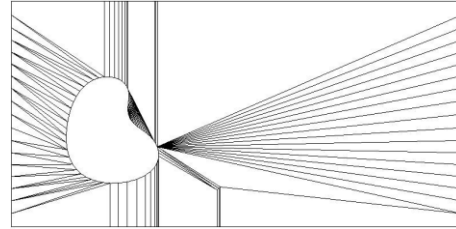
Figure 13: Corrected initial mesh.
