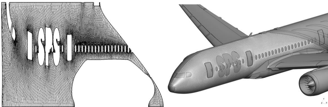
Figure 2: Surface mesh of a model face. View of the mesh in the parameter plane (left) and on \mathbb{R}^3 . where u \in [0, \pi] is the inclination and v \in [0, 2\pi[ is the azimuth. At the poles, i.e. when u = 0 or u = \pi ,
