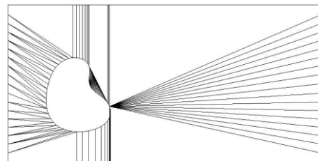
Figure 10: The initial mesh for the surface presented in 9 represented in the parameter plane.
