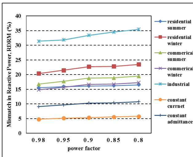
Figure 5. Reactive demand response mismatch with 10% reduction.
