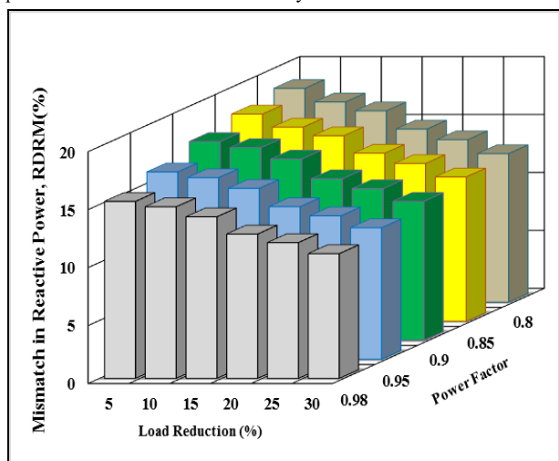
Figure 2. Active demand response for commercial winter load with different power factor and load reduction at day time.
