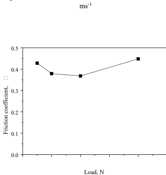
Fig. 5 Friction coefficient as a function of applied load under dry sliding condition at sliding velocity of 0.64 ms -1
