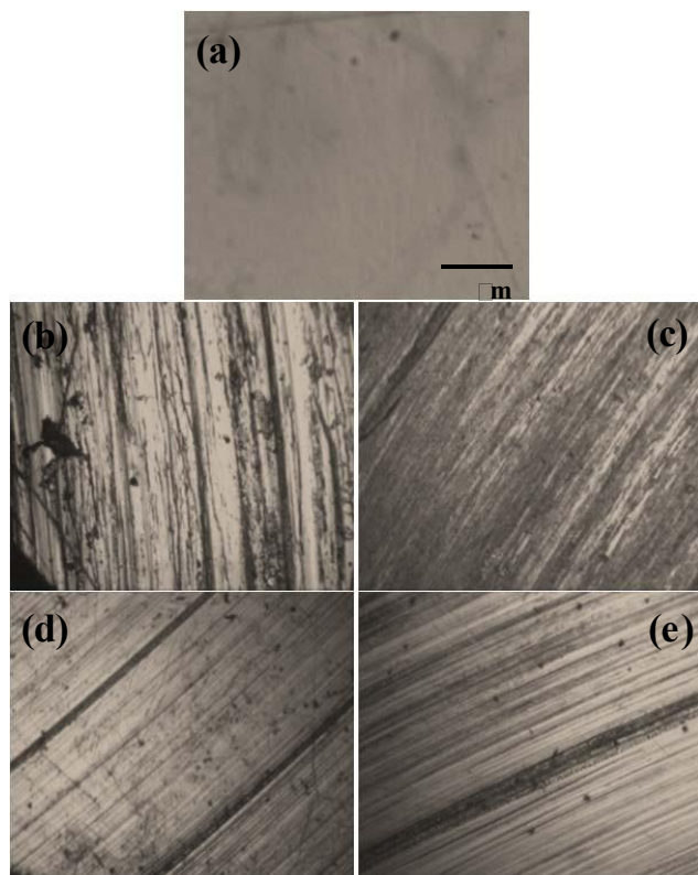
Fig. 9 Optical micrograph of worn surfaces a) before wear, b) 5 min in dry condition, c) 120 min in dry condition, d) 5 min in wet condition and e) 120 min in wet condition
