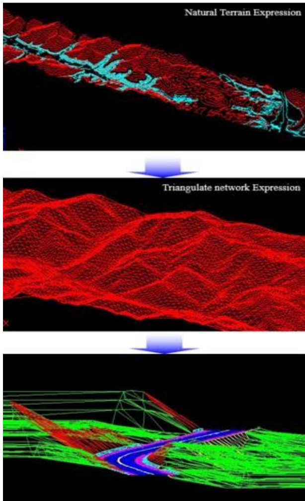
Fig. 4 Earthwork modeling process of natural terrain
