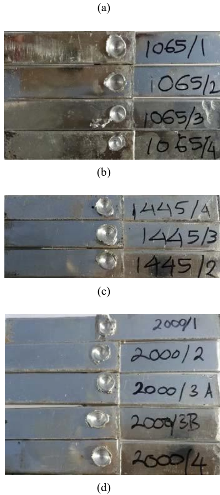
Fig. 10 FSSW sheets welded at different rotational speed (a) 760 RPM, (b) 1065 RPM, (c) 1445 RPM, (d) 2000 RPM
