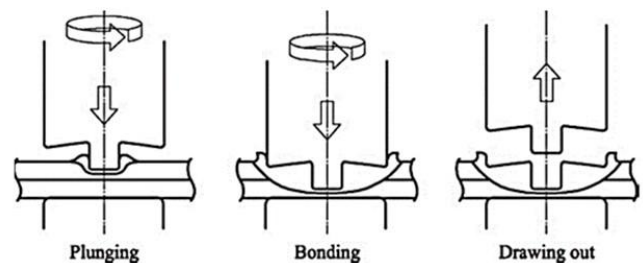
Fig. 1 A schematic illustration of the spot friction welding process [8]
