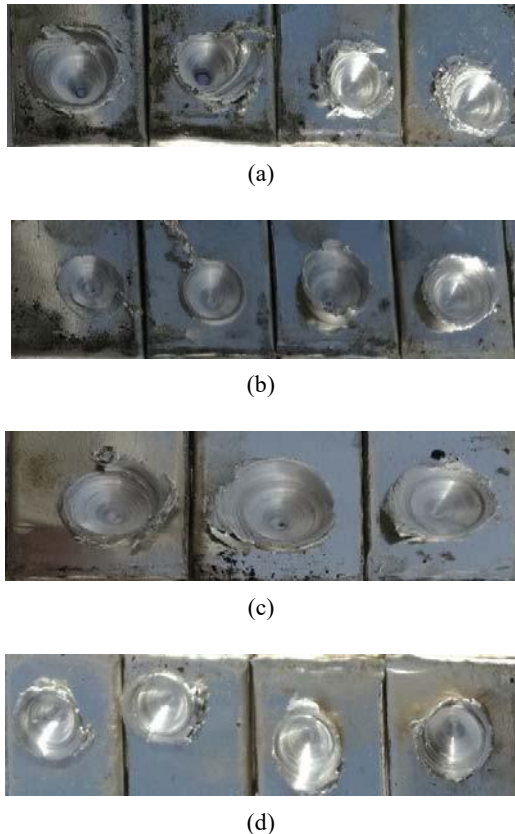
Fig. 12 Shape FSSW welded point at different rotational speeds (a) 760 RPM, (b) 1065 RPM, (c) 1445 RPM, (d) 2000 RPM
