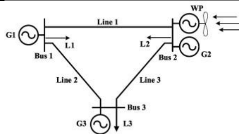
Figure 2 Modified 3-bus test system [3], [37].
