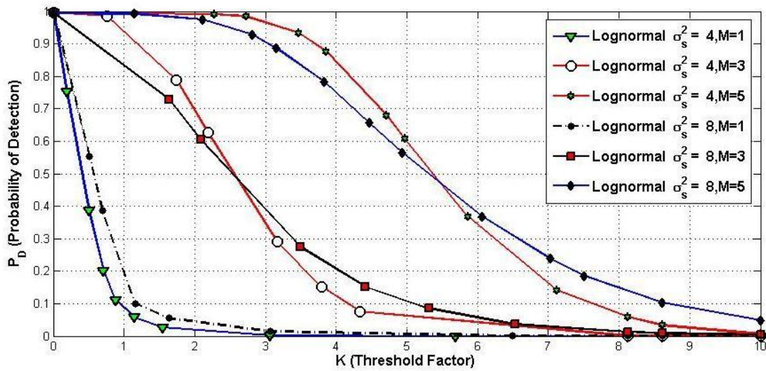
Fig.6 The impact of K on the probability of detection ( P_D ) when \sigma_p^2 \leq 8 .
