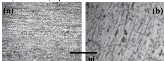
Fig. 5 Microstructure of Al-19Si automotive alloy before corrosion (a) polished (b) etched
