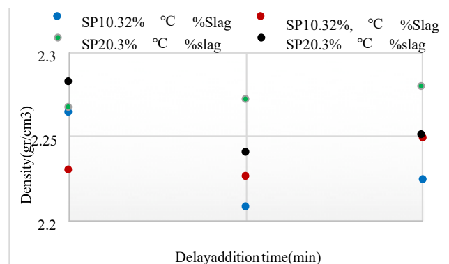
Fig. 4 Effect of heat stimulation and delayed addition of SP with 30% slag on fresh density of mortar
