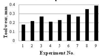
Fig. 9 Tool wear of undamped boring bar
