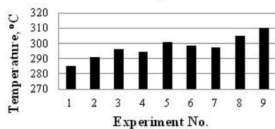
Fig. 6 Temperature of undamped boring bar
