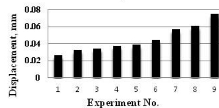
Fig. 3 Displacement of undamped boring bar
