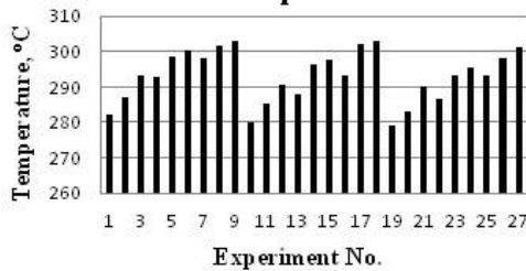
Fig. 7 Temperature of damped boring bar
