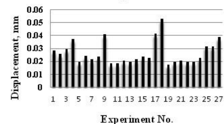
Fig. 4 Displacement of damped boring bar
