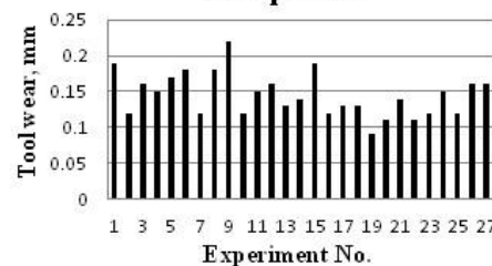
Fig. 10 Tool wear of undamped boring bar
