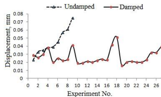
Fig. 5 Displacement of damped and undamped bar
