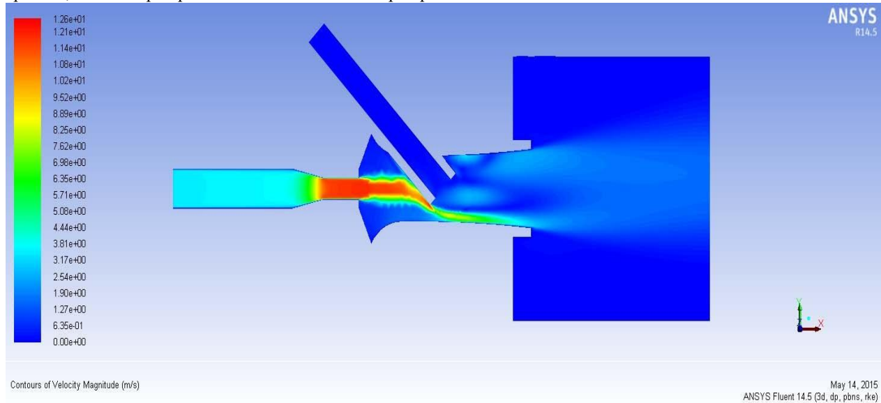
Fig. 8 Motive fluid deflection for pump where \alpha=45^\circ
