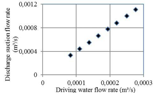
Fig. 4 Relation between discharge suction flow rate and driving water flow rate
