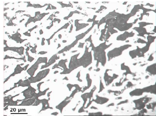
Fig. 6 The microstructure of the porous stainless steel disc
