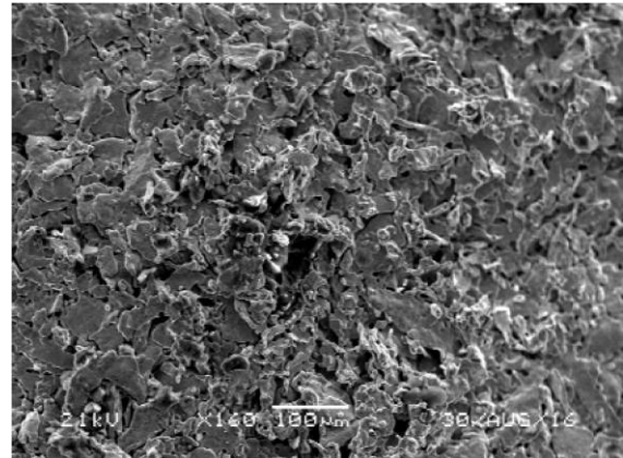
Fig. 2 A scanning electron micrograph of the fractured surface of a test specimen
