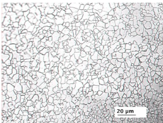
Fig. 5 The microstructure of the solid iron tube in the HAZ
