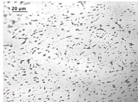
Fig. 7 The microstructure of the porous stainless steel in the heat affected zone
