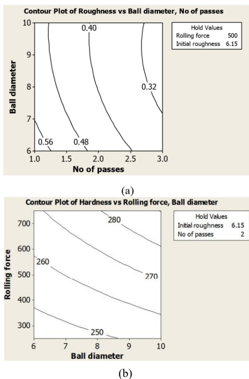
Fig. 8 Three dimensional plot of (a) surface roughness (b) surface hardness
