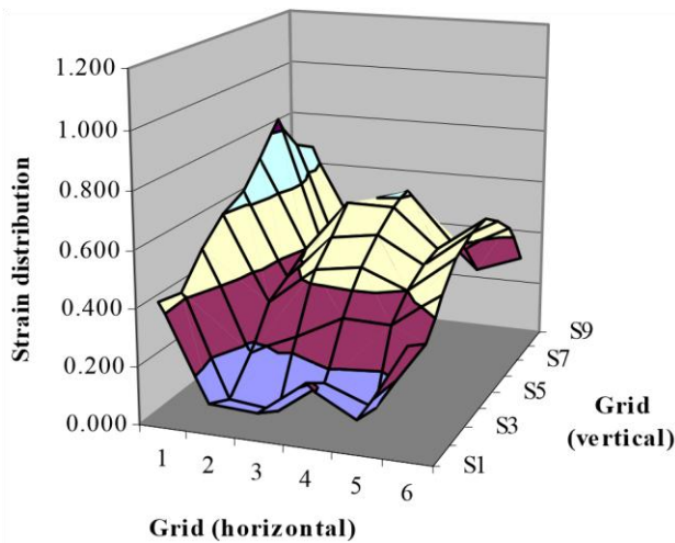
Fig. 7 Actual strain distribution pattern observed due to deformation of grid at the end of Stage 3
