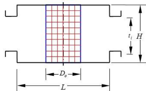
Fig. 1 Initial configuration of Die-Billet geometry
