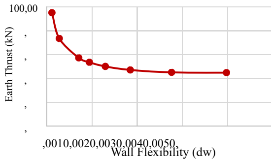
Fig. 5 Effect of wall flexibility on earth pressure by present 2-DOF model
