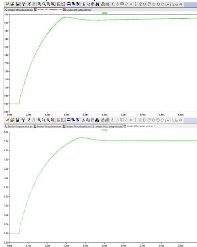
Figure 7.2: Output voltage for the improved converter (top) and for the conventional Flyback (bottom).
