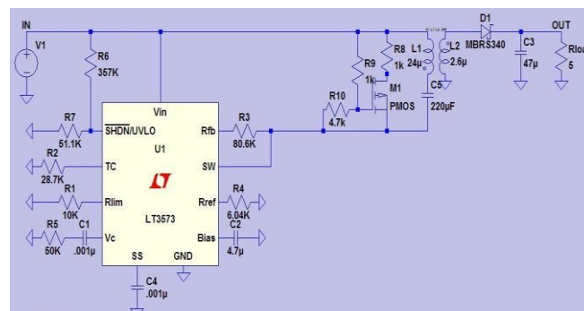
Fig. 1: Implemented Improved Flyback converter
