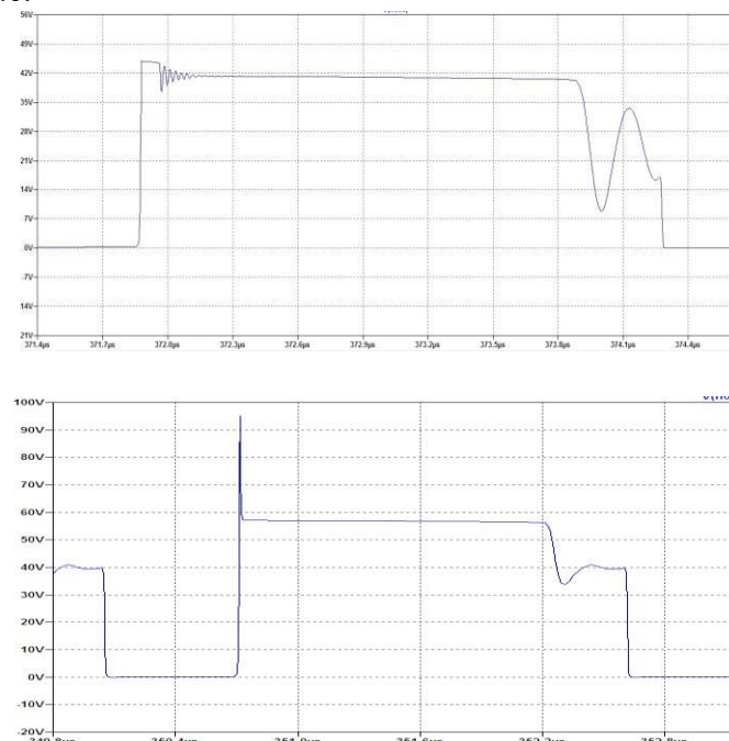
Figure 7.1: Primary mosfet voltage for the improved converter (top) and for the conventional Flyback (bottom).
