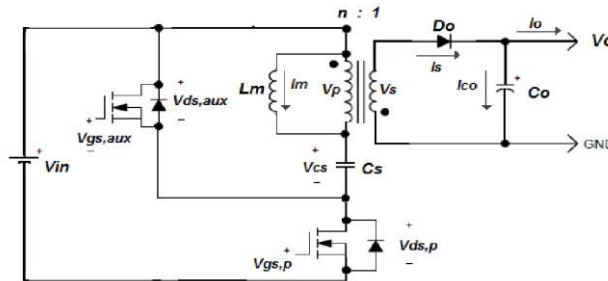
Fig. 1: Implemented Flyback converter
