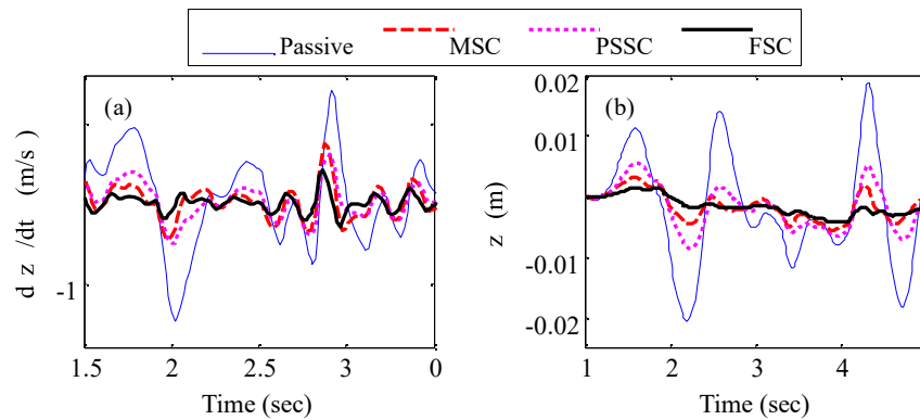
Fig. 7 Passenger seat response (a) acceleration (b) displacement
