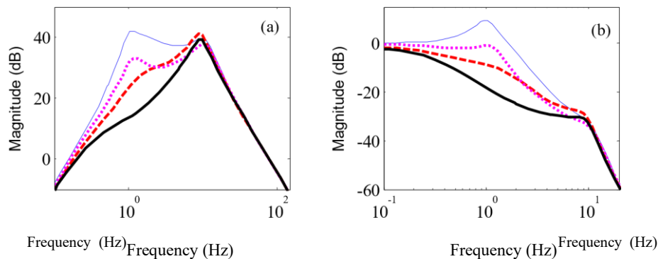
Fig. 13 Bode plot (a) Passenger seat acceleration (b) Passenger seat displacement
