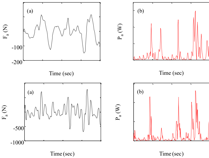
Fig. 9 Main suspension controlled (a) Damping force supplied by ANFIS controller (b) Power consumed by ANFIS controller Fig. 10 Passenger seat suspension controlled (a) Damping force supplied by ANFIS controller (b) Power consumed by ANFIS controller
