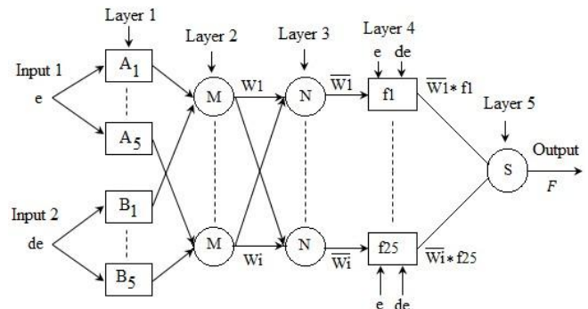
Fig. 3 Five layer ANFIS structure for active quarter car model
