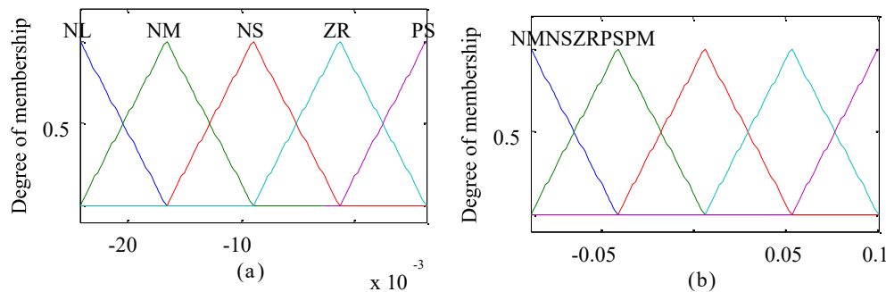
Fig. 4 Membership functions for (a) error signal ( ), (b) derivative of error signal ( )
