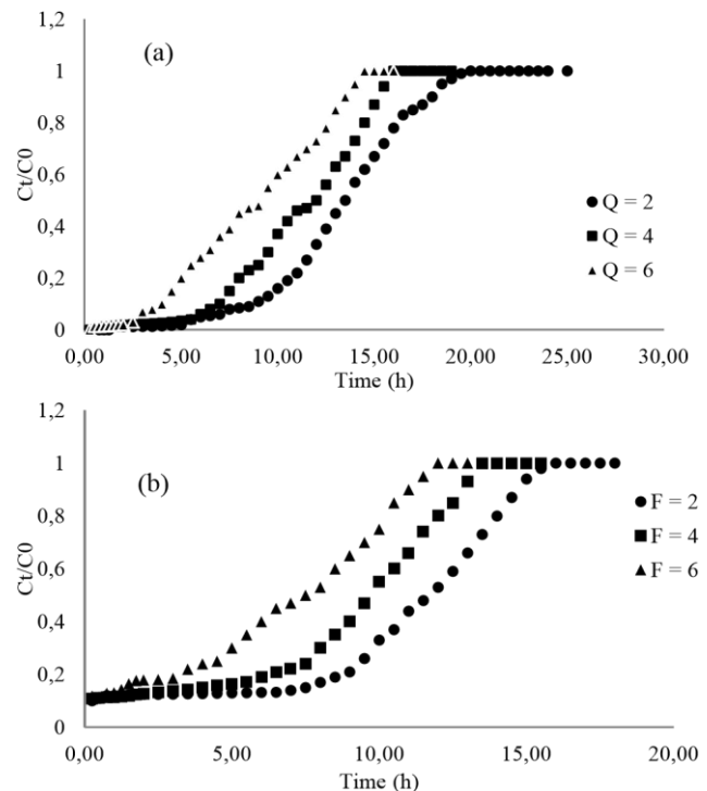
Fig. 2 Breakthrough curves for biosorption of Cu (A) and Mn (B) ions at different flow rates
