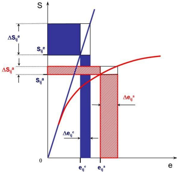
Fig. 2 Graphical representation of the incremental Neuber rule
