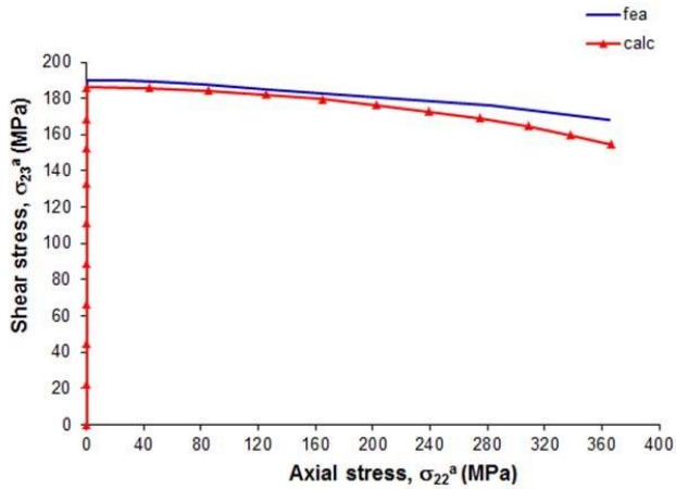
Fig. 4 Comparison of the calculated and FEM determined stress paths for the non-proportional torsion-tension load path
