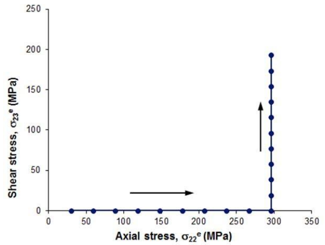
Fig. 6 The non-proportion tension-torsion load path
