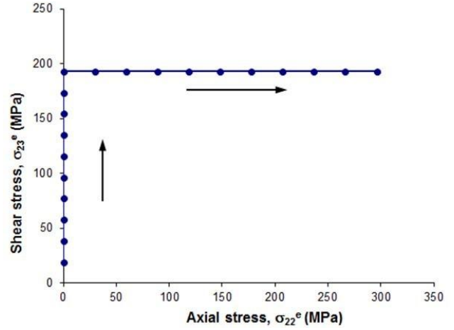
Fig. 3 The non-proportion torsion-tension load path
