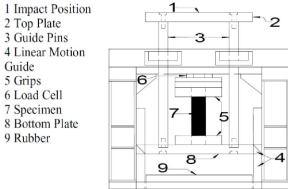
Fig. 2 Schematic view of the fabricated tensile impact rig [8]
