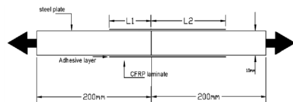
Fig. 1 Schematic view of the CFRP-steel double-strap specimen
