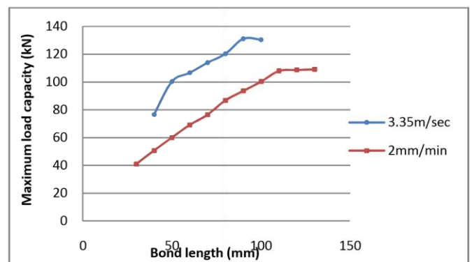
Fig. 6 Ultimate joint capacity vs. bond length for the two load rates
