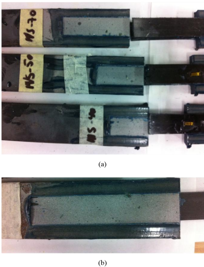
Fig. 5 De-bonding failure for the quasi-static specimens: (A) less than the effective bond length, (B) beyond the effective bond length
