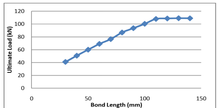
Fig. 3 Load vs. bond length for the quasi-static specimens
