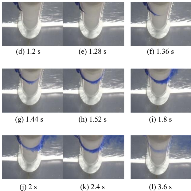
Fig. 6 Ink Dispersion Technique: Flow of pigmentation under influence of entrainment
