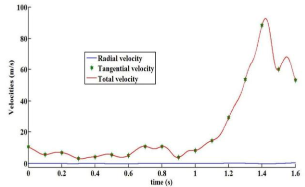
Fig. 7 Total, Tangential, Radial Velocity of Ink tip versus time
