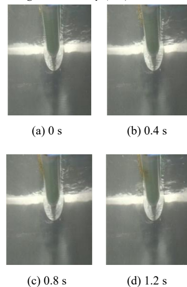
Fig. 8 Particle Image Velocimetry: Flow of seeded particles at different time stamps
