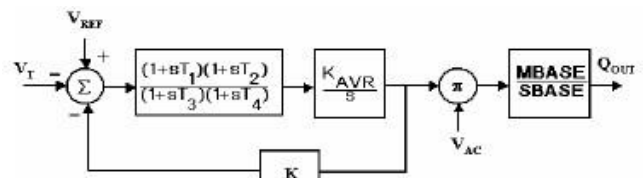
(b) Reactive power control function of STATCOM/SMES compensator
