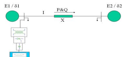
Fig. 4 General model of the proposed STATCOM/SMES compensator
