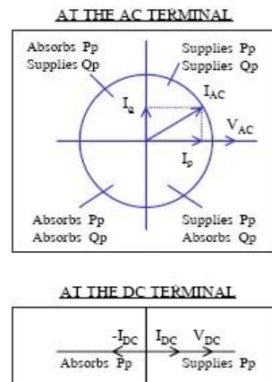
Fig. 6 Benefits of STATCOM with SMES
