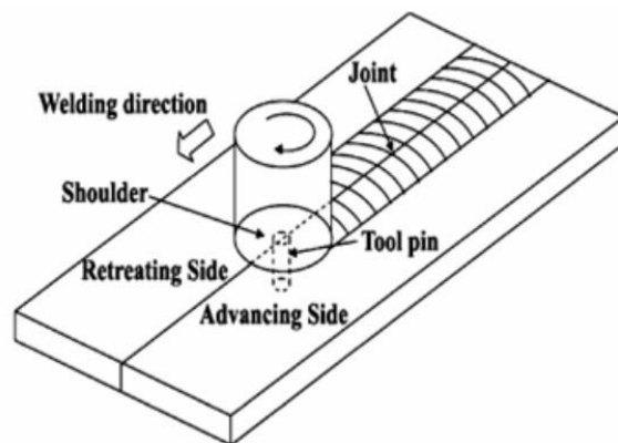
Fig. 1 Friction stir welding
