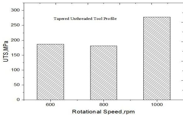
(a) UTS vs Rotational speed for Tapered Unthreaded tool (b) UTS vs Rotational speed for Tapered threaded tool
