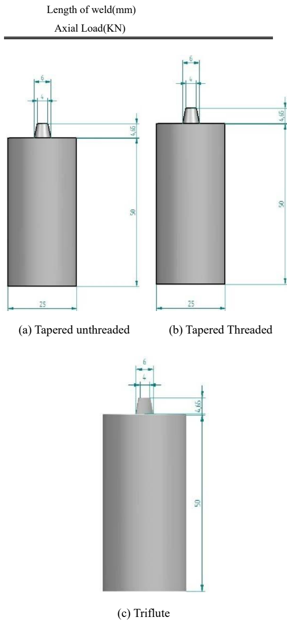
Fig. 4 Different tool profiles used
