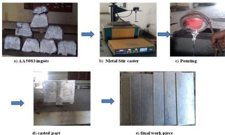
Fig. 2 Step by step procedure of material preparation
