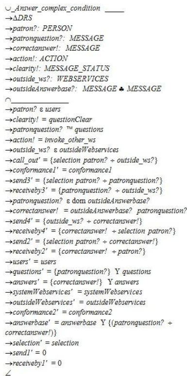
Fig. 9 Answer_complex_condition schema
