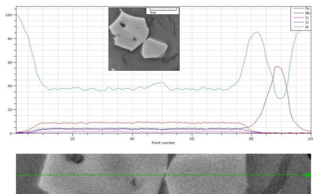
Fig. 9 The Al_{15}(FeMnCr)_3Si_2 identification using phase line EDX analysis, etc. 0.5 % HF
