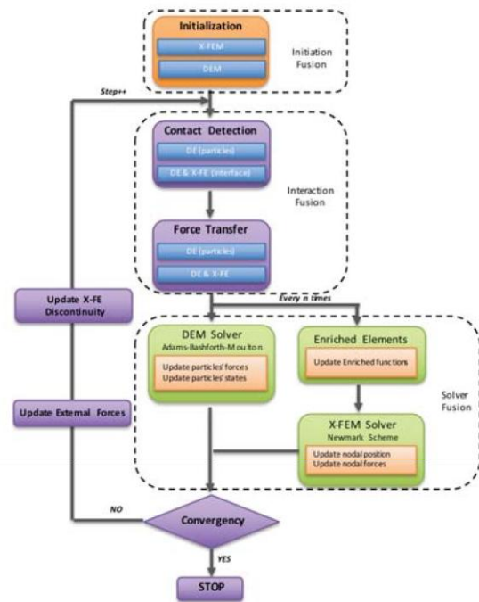
Fig. 3 The solution procedure of X-FE-DEM
