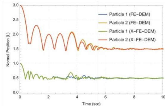
Fig. 14 Comparison between the response of the discontinua in FE-DEM and X-FE-DEM for case II
