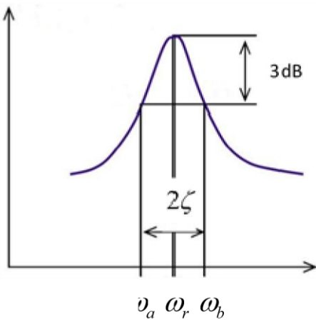
Fig. 3 Extracting natural frequencies of RC slabs A and B from FRF
