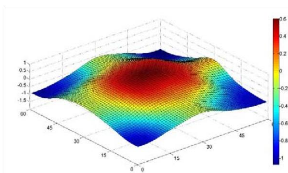
Mode Shape 3
