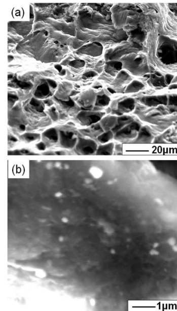
Fig. 9 SEM micrograph of the fractured surfaces of tensile specimens
