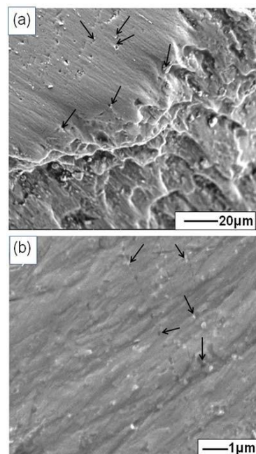
Fig. 10 SEM micrograph of polished longitudinal section of failed tensile specimen of forged composite AM4P2, just below the fracture surface at (a) lower and (b) higher magnifications
