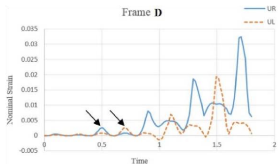
Fig. 9 Strain diagram for the upper cables in model D
