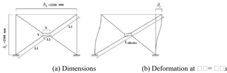
Fig. 5 Delayed wire-rope bracing using middle plate
