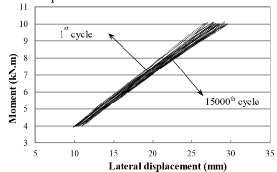
Fig. 9 Cyclic response of flexi-wall from 1 to 15000 cycles
