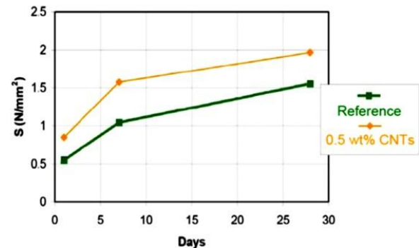
Fig. 3 Dissipated Energy Density vs. days of curing [7]
