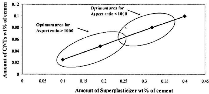
Fig. 7 Determination of the optimum amount of CNTs and the correspondingly required amount of superplasticizer depending on the aspect
