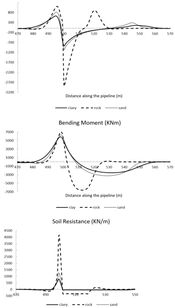
Fig. 13 Vertical displacements, shear forces, bending moments and soil resistance forces for the considered soil conditions, in the area near the fault trace; intersection with a normal fault
