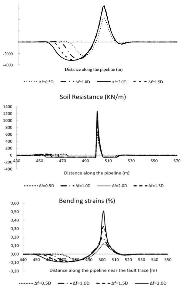
Fig. 9 Vertical displacements, shear forces, bending moments, soil resistance forces for upward and downward displacement and bending strains along the length of the pipeline, in the area near the fault trace; intersection with a reverse fault
