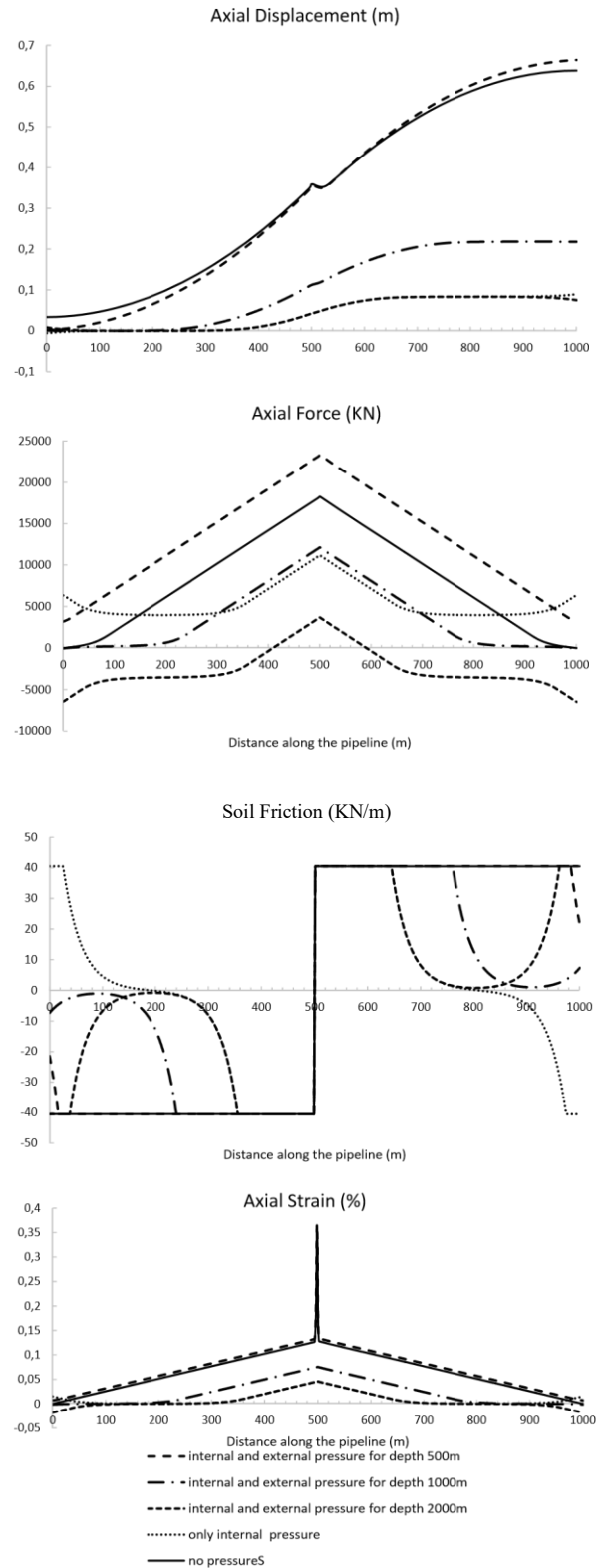
Fig. 10 Axial displacement, axial forces, soil friction forces and axial strains along the length of the pipeline for the considered pressure states; intersection with a normal fault
