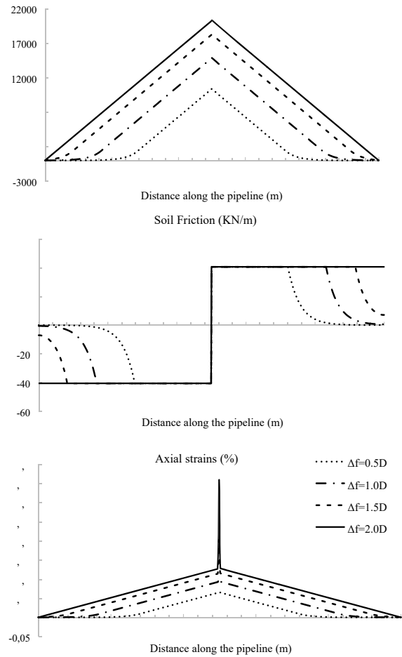
Fig. 6 Axial displacement, axial force, soil friction forces and axial strain along the length of the pipeline for the considered fault displacements; intersection with a normal fault
