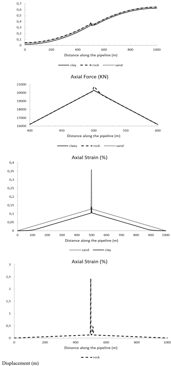
Fig. 12 Axial displacement, axial forces, soil friction forces and axial strains along the length of the pipeline for the considered soil conditions; intersection with a normal fault
