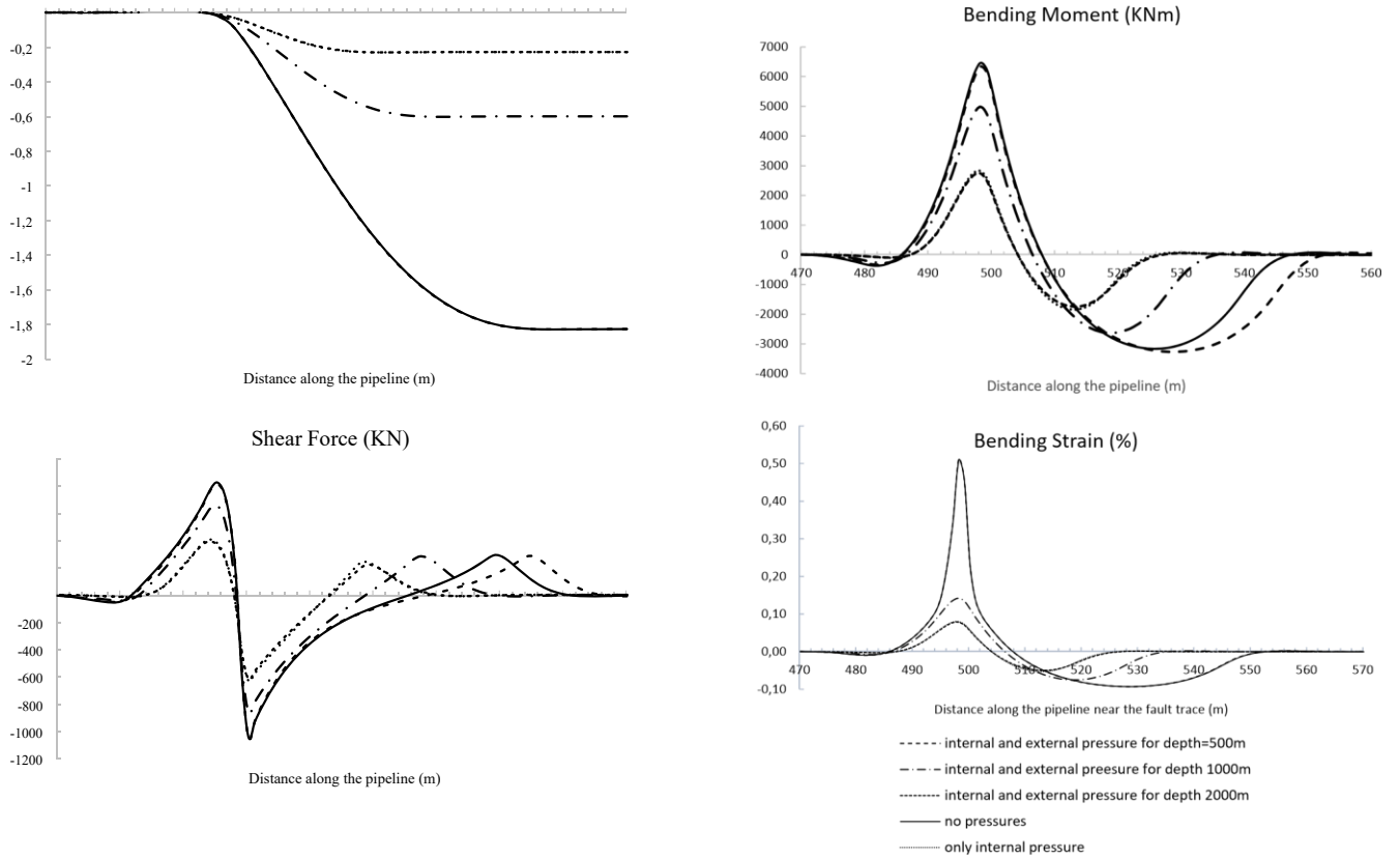
Fig. 11 Vertical displacements, shear forces, bending moments, soil resistance forces and bending strains along the length of the pipeline, for the considered pressure states, in the area near the fault trace; intersection with a normal fault
