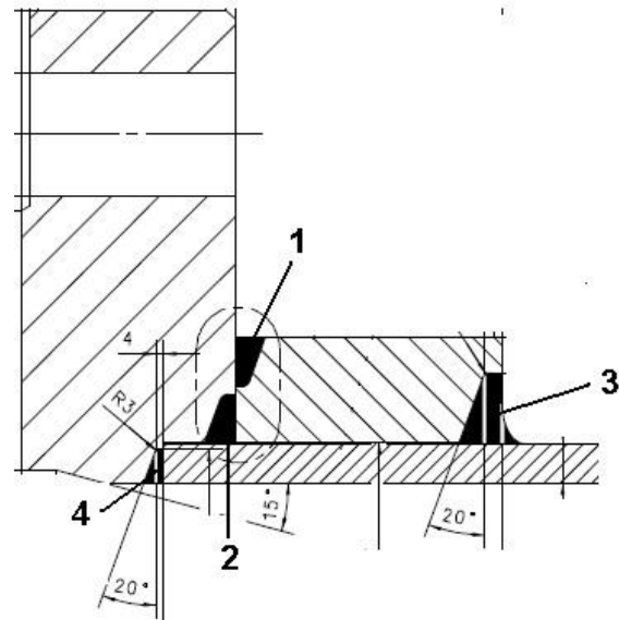
Fig. 7 Assembly drawing of the plate-pipe system
