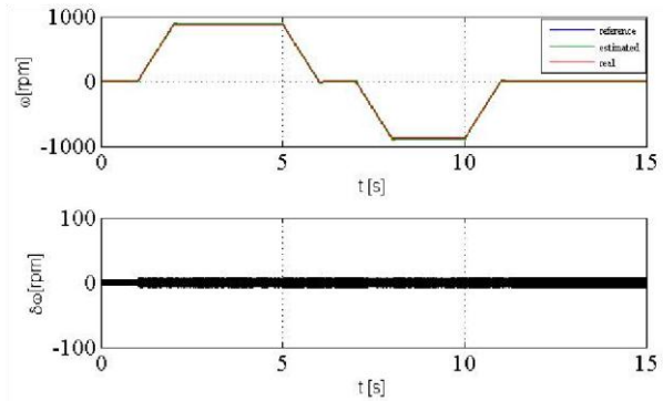
Fig. 7 R_r variation to double of rated value
