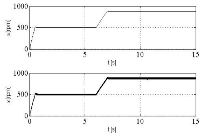
Fig. 2 Real and estimated speed in acceleration test
