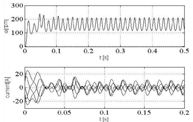
Fig. 1 Running up test without any applied control
