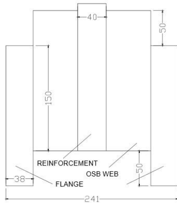
Fig. 3 Specimen dimensions
