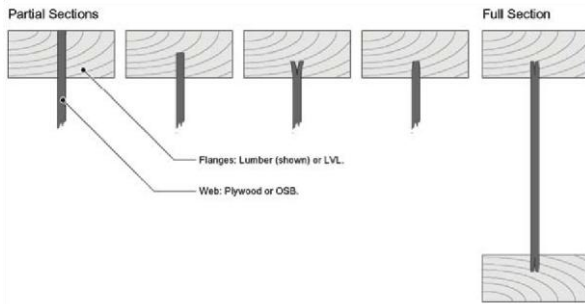
Fig. 2 Web-to-flange joints models and materials
