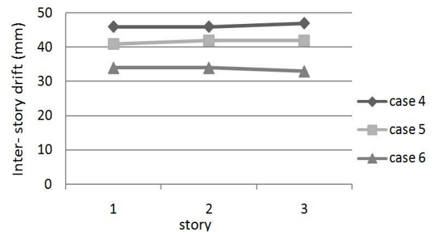
Fig. 27 The maximum displacement between floors under rectangular impact load
