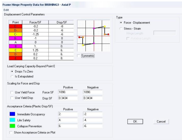
Fig. 20 The brace plastic joint of the third floor
