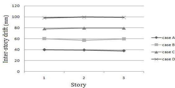
Fig. 17 Displacement between floors
