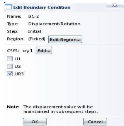
Fig. 9 Boundary conditions of bracing system
