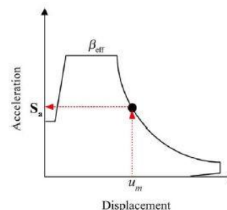
Fig. 3 Response spectrum of displacement- acceleration (ADRS)
