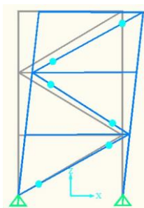
Fig. 23 Formation of Plastic Joints in the Structure VI. STEEL FRAME BEHAVIOR WITH BUCKLING-RESTRAINED BRACES UNDER IMPACT LOAD
