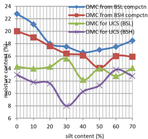
Fig. 5 Variation of OMC for maximum UCS with A-3 soil content at BSL and BSH Energy
