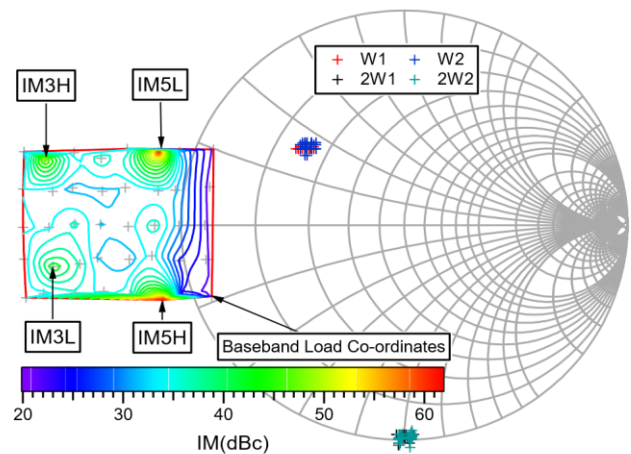
Fig. 10 Experimentally measured IM linearity contours as a function of IF reflection coefficient ( \Gamma_L ) for a class-J emulated RF impedance environment
