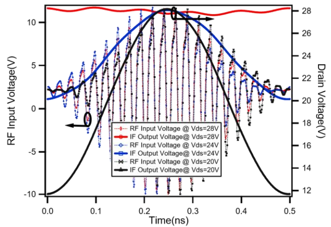
Fig. 8 Experimentally measured dynamic IF voltage envelopes in-phase with input RF voltages for the three cases considered
