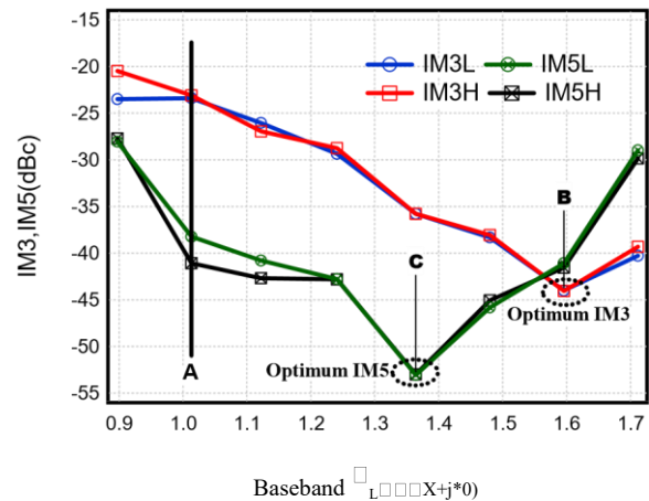
Fig. 6 Experimentally measured IM3 and IM5 linearity trade-off as a function of baseband reflection coefficient ( \Gamma_L )
