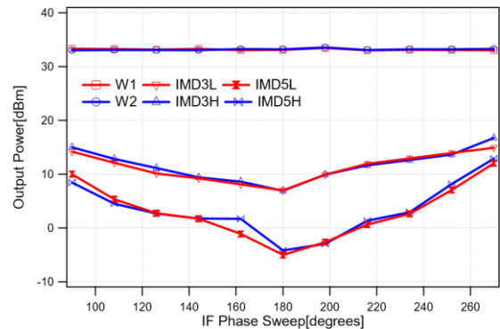
Fig. 2 Experimentally measured baseband impedances at 2MHz tone spacing using active IF load-pull with RF terminated to 50Ω
