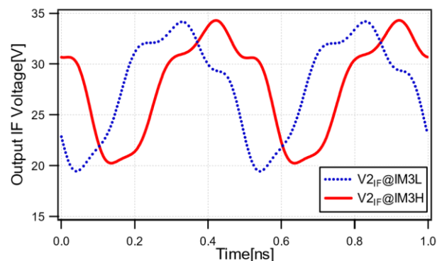
Fig. 11 Experimentally measured baseband voltages that resulted for the best IM3 linearity performance under class-J mode of operation
