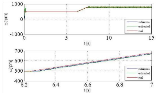
Fig. 1 Real and estimated speed in acceleration test
