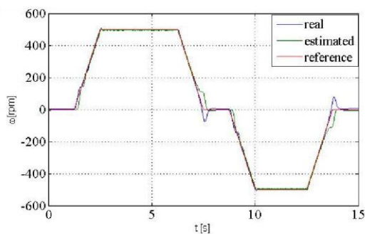
Fig. 6 R_r variation to double of rated value
