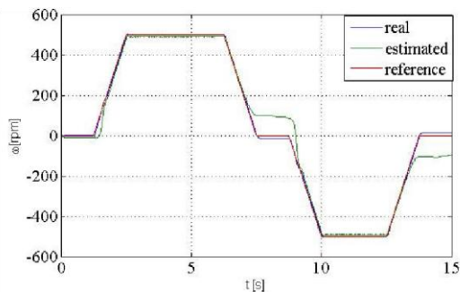
Fig. 5 L_m variation to half of rated value
