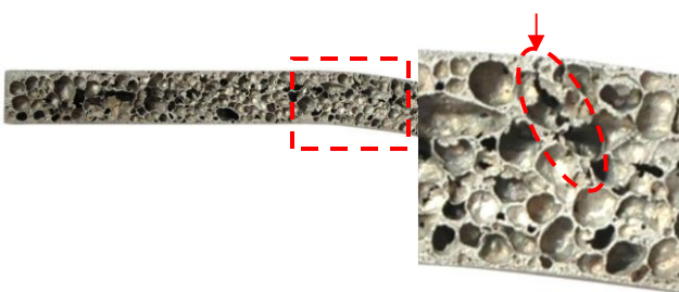
Fig. 7 Section macro views of bended specimen in 640 °C and crack formation on the top surface
