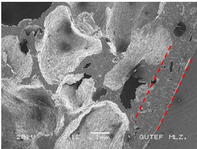
Fig. 6 Tensile region of bended specimen in 656°C
