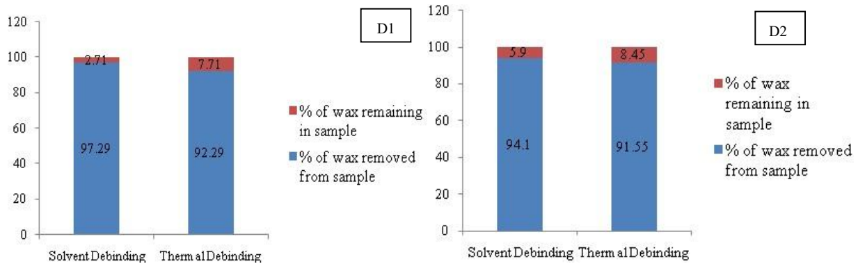
Fig. 9 Solvent and thermal debinded Sample D1 and D2
