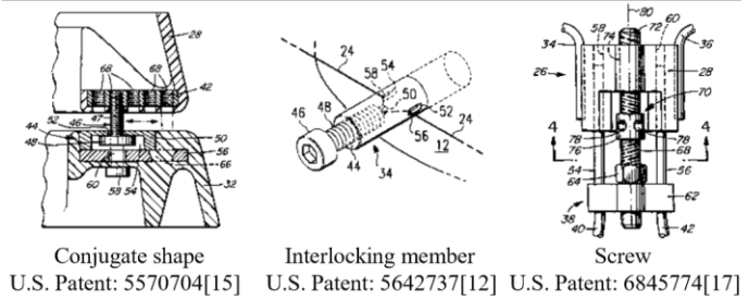
Conjugate shape U.S. Patent: 5570704[15] Interlocking member U.S. Patent: 5642737[12] Screw U.S. Patent: 6845774[17]
