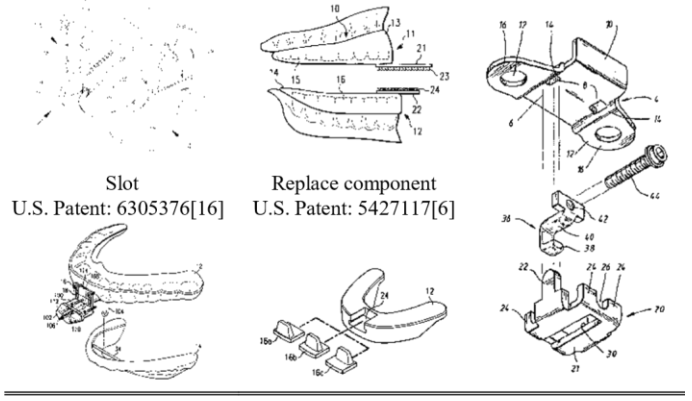
Conjugate shape U.S. Patent: 5570704[15] Interlocking member U.S. Patent: 5642737[12] Screw U.S. Patent: 6845774[17]
