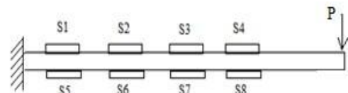
Fig. 2 Schematic showing numbering of strain gauges
