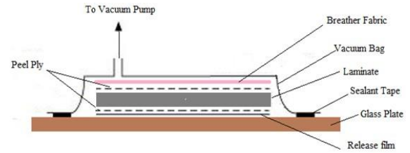
Fig. 1 Layup sequence for vacuum bagging
