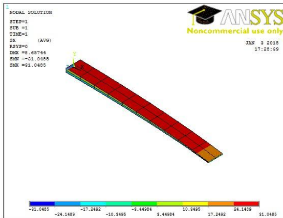
Fig. 6 Stress plot at Load P = 19.62 N
