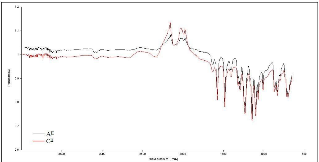
Fig. 8 FTIR Spectroscopy of PSU/Sep. nanocomposites prepared with DMAC-Chloroform solvent mixture
