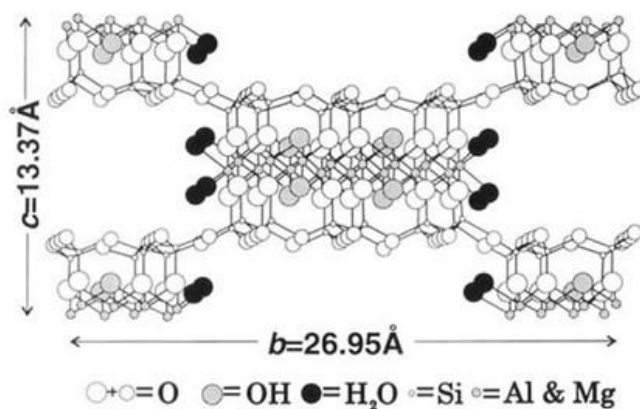
Fig. 1 Structure of sepiolite [10]
