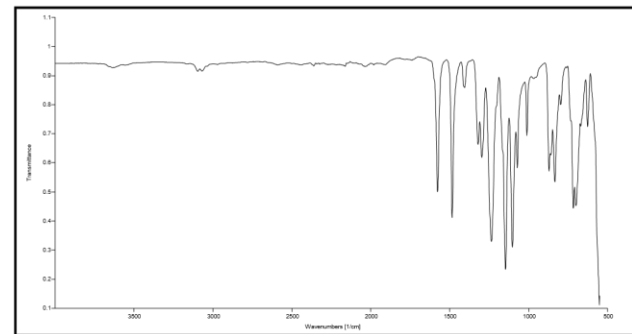
Fig. 5 Polysulfone
