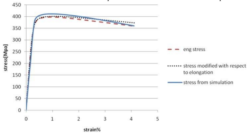
Fig. 7 Stress-strain curves obtained from experiments and simulations for notched specimen r=10 mm
