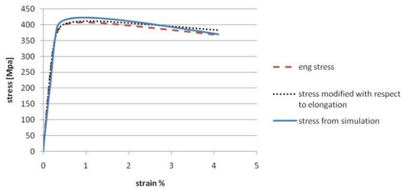
Fig. 8 Stress-strain curves obtained from experiments and simulations for notched specimen r=12 mm
