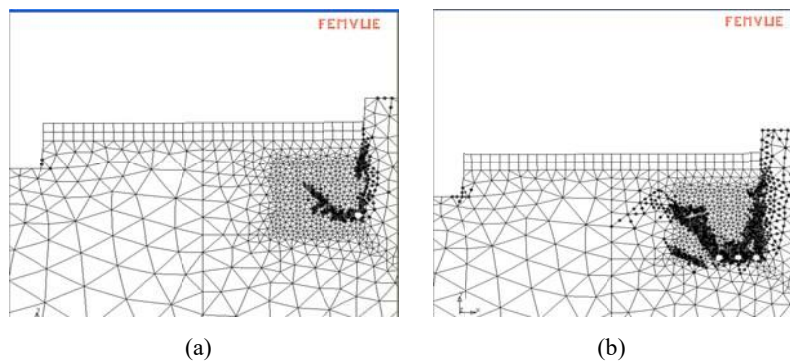
Fig. 11 Plastic point distribution for U-shape sliding surfaces
