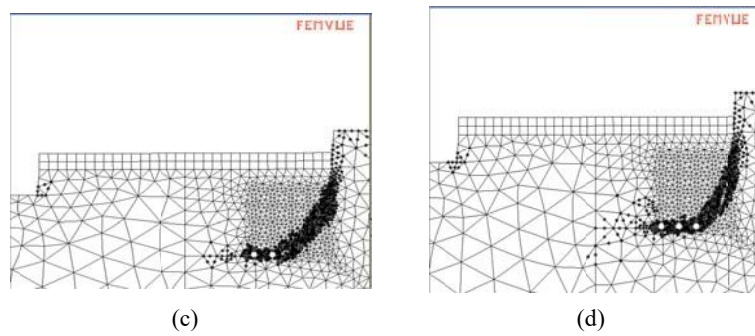
Fig. 10 Plastic point distribution for smooth sliding surfaces
