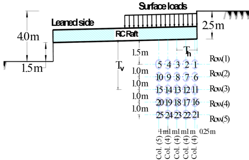
Fig. 4 Alternative suggested locations of the micro-tunnels
