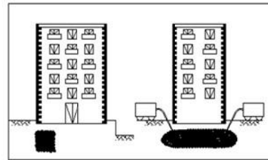
(g) Additional surface load gradual application (if needed) (h) Strengthen grouting for soil stabilization
