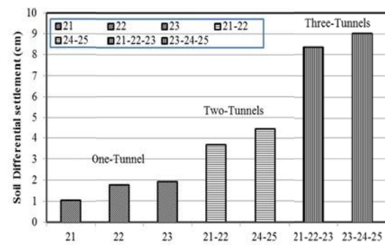
Fig. 6 Effect of tunnel location on soil differential settlement under tilted building
