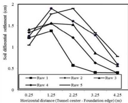
Fig. 8 Effect of tunnel location ( T_H ) on soil differential settlement Fig. 9 Effect of micro-tunnels number on soil differential settlement
