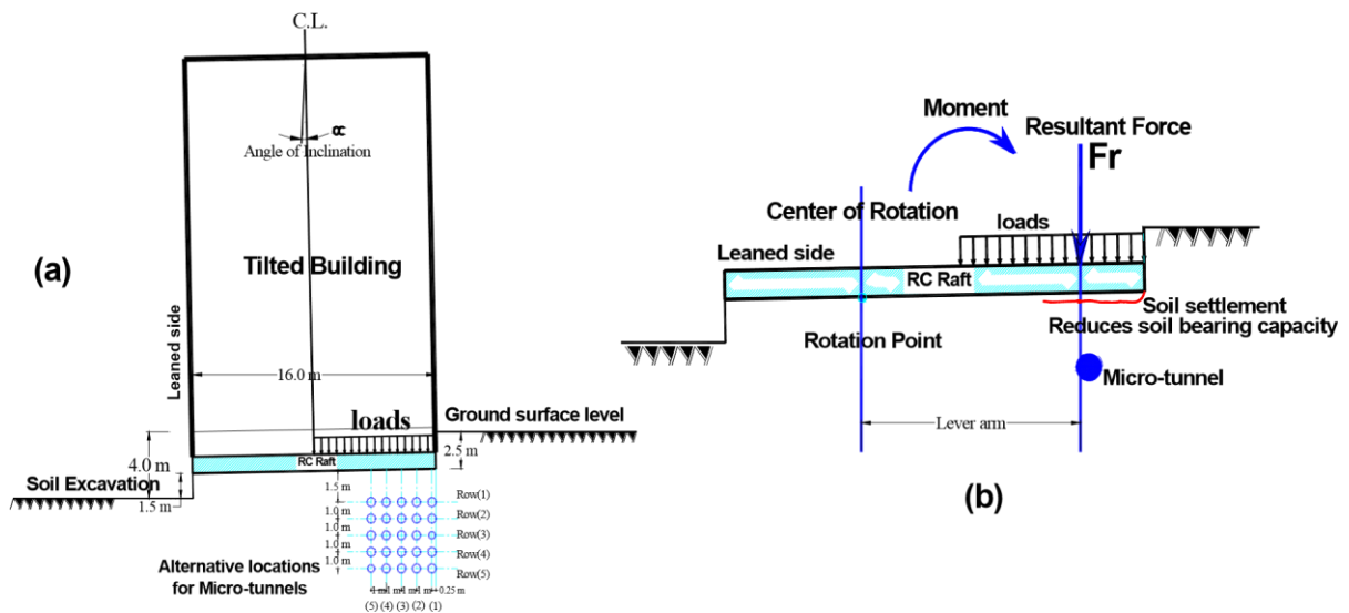
Fig. 3 Details of tilted building (case study) and the forces and stresses applied on its raft foundation
