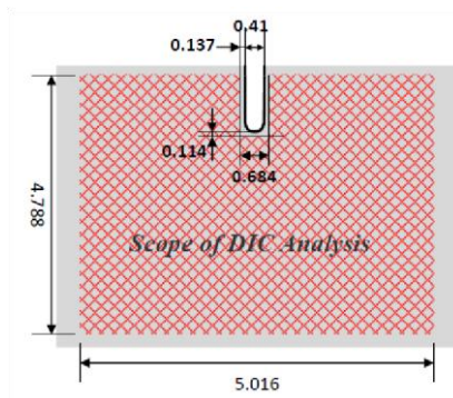
Fig. 5 Sketch of DIC measuring range
