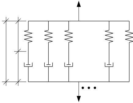
Fig. 2. Generalized Maxwell chain consisting of P viscoelastic units and elastic spring.
