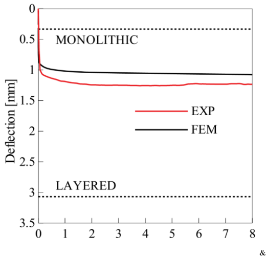
Fig. 6. Comparison of deflection at the mid-point of one of the spans of a two-span simply supported beam with a symmetric layout of layers with thicknesses of glass layers 4 mm and PVB layer 0.38 mm, length of 1.4 m, the spans of 0.7 m, and the width of 0.1 m, under the uniform distributed loading of intensity f_z = 94.22 \text{ N/m} at the temperature T = 17.8^\circ\text{C} . (EXP: experimental data, FEM: response of finite element model of laminated glass beam in terms of deflections.)
